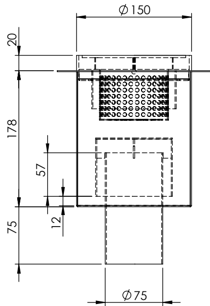
FRONT VIEW SCALE 1:5 @ A4
